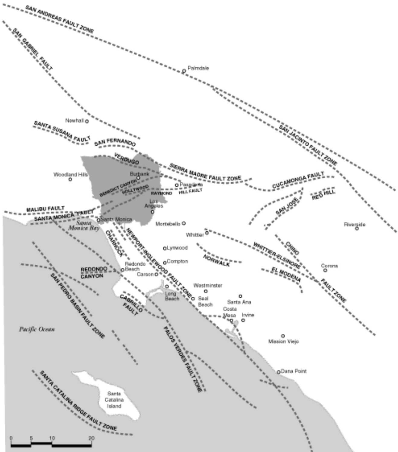
Figure 2-3 Major Faults in the Watershed Vicinity
