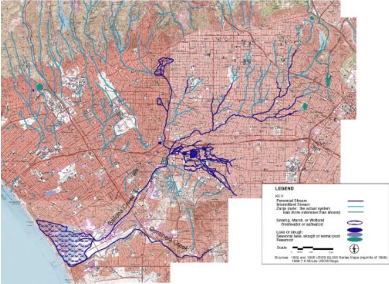
Figure 2-6 Historic Ballona Creek Watershed Drainage Area Overlay Map, 1896 and 1986 SOURCE: Braa, et al., 2001, Seeking Streams: A Landscape Framework for Urban and Ecological Revitalization in the Upper Ballona Creek Watershed
